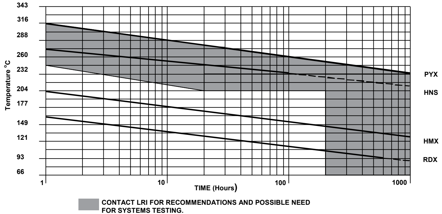
°C Operational Limits for Hollow Carrier Gun Systems
